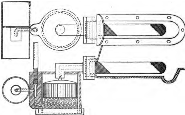
FIG. 156.—The Duryea Float Feed Carburettor or Sprayer.
